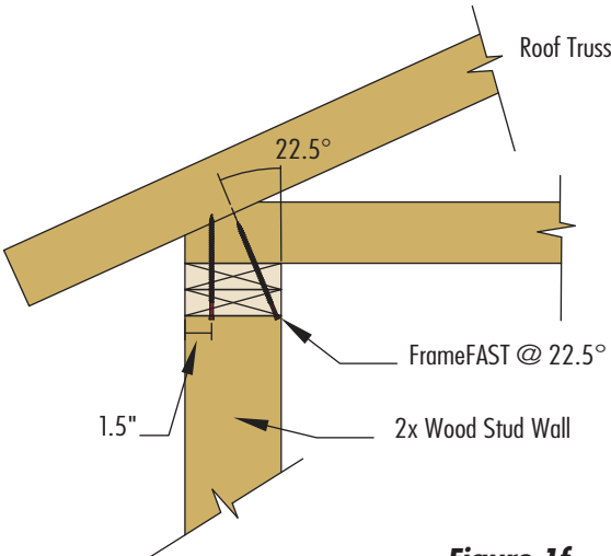
Figure 1f Two Screw Installation
