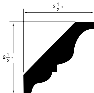
CROWN MOULDING WSCR19 - Top 2-1/2" x 2-1/2"
