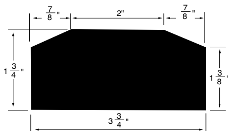
HANDRAIL - S.E. BOTTOM RAIL WSHR18 3-3/4"x1-3/4"
