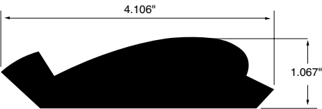
CROWN MOULDING WSCR4 4.106"x1.067"
