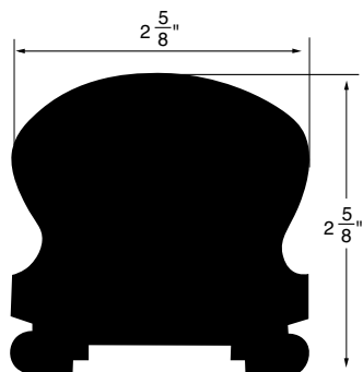
HANDRAIL WSHR13 2-5/8"x2-5/8"
