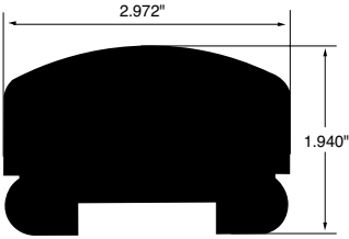
HANDRAIL WSHR7 2.972"x1.940"
