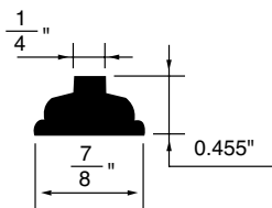
INTERIOR DOOR MOULDING WSD2 7/8"x0.455"
