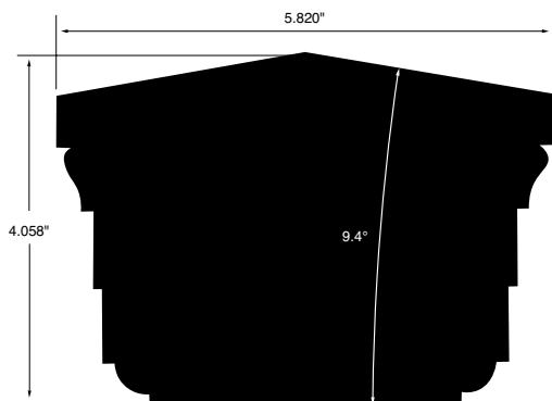
HANDRAIL WSHR1 5.820"x4.058"
