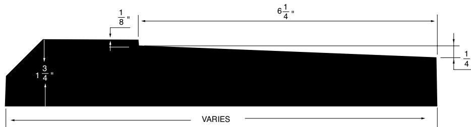
DOOR SILL WWS3 Width Varies x Thickness 1-3/4"
