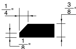
DOOR STOP WSDS2 1"x3/8"
