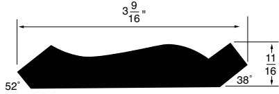
CROWN MOULDING WSCR26 3-9/16" x 2-11/16"
