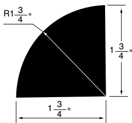
QUARTER ROUND WSQR1 2-1/2"x1-3/4"
