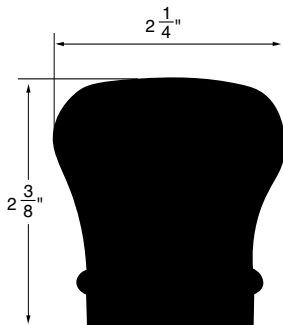
HANDRAIL WSHR5 2-1/4"x2-3/8"
