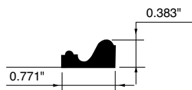
PANEL MOULDING WSPM24 0.771"x0.383"
