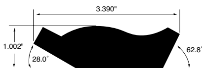
CROWN MOULDING WSCR23 3.390" x 1.002"
