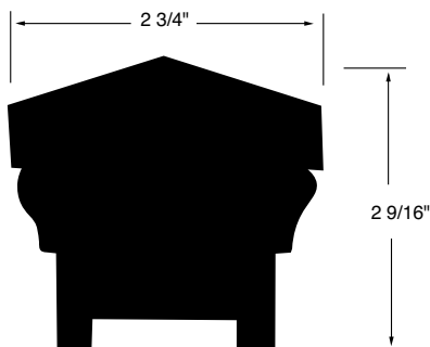
HANDRAIL WSHR3 2-3/4"x2-9/16"
