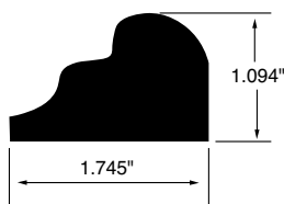
PANEL MOULDING WSPM8 1.745"x1.094"
