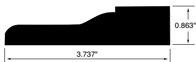
CASING WSCA12 3.737"x0.863"
