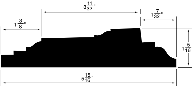
CASING WSCA51 5\frac{15}{16}" \times 1\frac{5}{16}"
