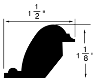
CAP MOULDING WSCM17 1-1/2"x1-1/8"
