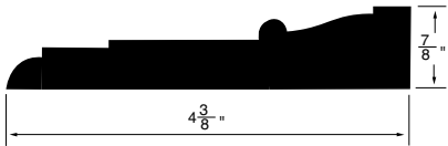
CASING WSCA19
