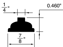
PANEL MOULDING WSPM23 7/8"x0.460"
