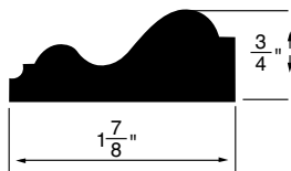
PANEL MOULDING WSPM20 1-7/8"x3/4"
