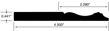
BASEBOARD WSBB10 4.500"x0.441"
