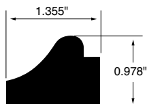
PANEL MOULDING WSPM38 1.355"x0.978"
