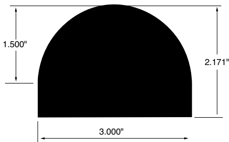
HALF ROUND WSHR5 3.000"x2.171"
