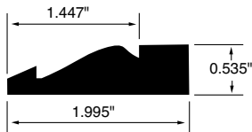
PANEL MOULDING WSPM32 1.995"x0.535"
