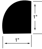
QUARTER ROUND WSQR3 1"x1"
