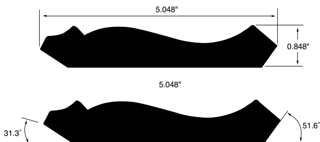
CROWN MOULDING WSCR7 5.048" x 0.848"
