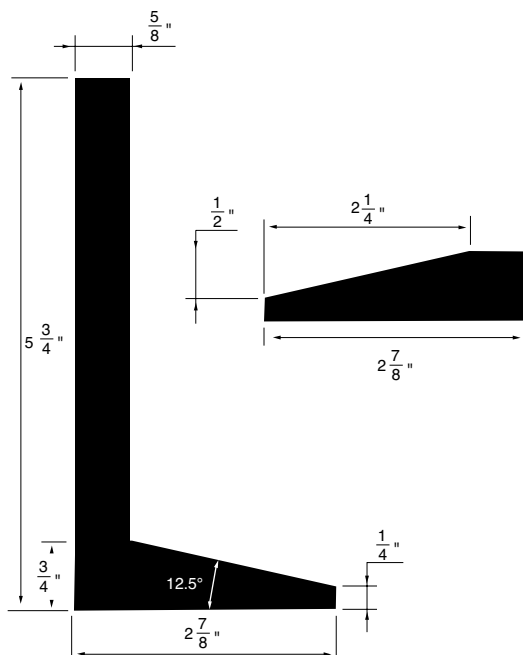
WINDOW SILL WWS2 2-7/8 x 5-3/4"
