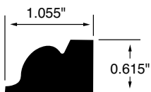
CAP MOULDING WSCM25 1.055"x0.615"
