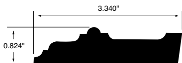
CASING WSCA4 3.340"x0.824"
