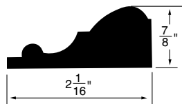
PANEL MOULDING WSPM6 2-1/16"x7/8"
