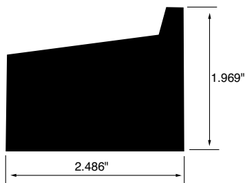
WINDOW SILL WWS1 2.486" x 1.969"
