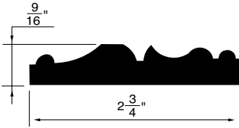
CASING WSCA48 2\frac{3}{4}" \times \frac{9}{16}"
