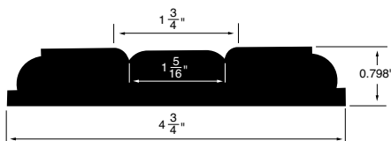
CASING WSCA30 4-3/4" x 0.798"
