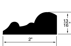
PANEL MOULDING WSPM1 2"x13/16"
