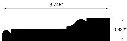
CASING WSCA57 3.745"x0.822"
