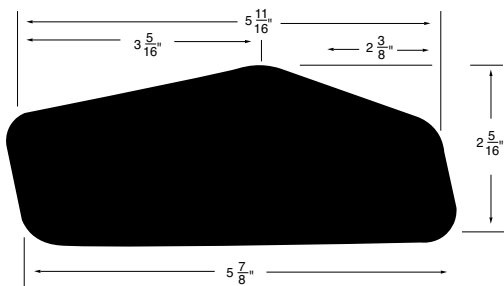
HANDRAIL WSHR4 5-7/8"x2-5/16"
