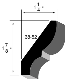
CROWN MOULDING WSCR22 1-1/4" x 1-7/8"
