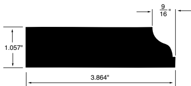
BASEBOARD WSBB1 3.864"x1.057"
