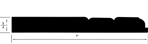
BASEBOARD WSBB13 7"x3/4"
