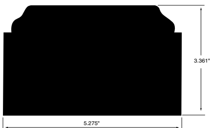
HANDRAIL WSHR6 5.275"x3.361"
