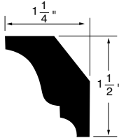
CROWN MOULDING WSCR27 1-1/4" x 1-1/2"
