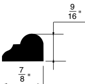
PANEL MOULDING WSPM20 7/8"x9/16"
