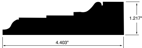
CASING WSCA1 4.403"x1.217"
