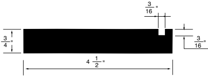
BASEBOARD WSBB11 4-1/2"x3/4"
