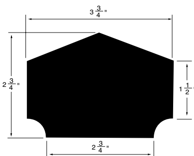
HANDRAIL - S.E. TOP RAIL WSHR16 3-3/4"x2-3/4"
