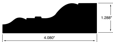
CASING WSCA41 4.080"x1.288"
