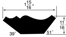
CROWN MOULDING WSCR27 1-15/16" x 1 11/16"
