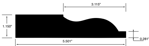
BASEBOARD WSBB3 5.501"x1.150"
