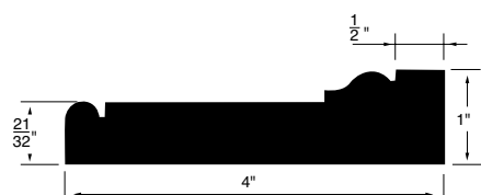
CASING WSCA11 4"x1"
