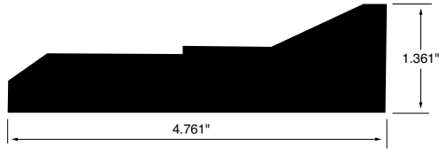
CASING WSCA47 4.761"x1.361"
