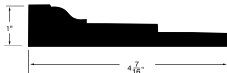
CASING WSCA27 4-7/16" x 1"
