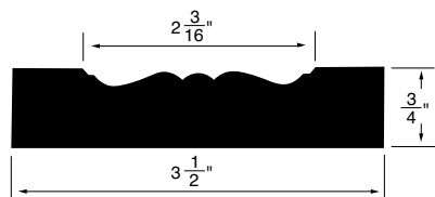
CASING WSCA42 3-1/2"x3/4"
