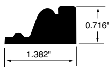
PANEL MOULDING WSPM25 1.382"x0.716"
