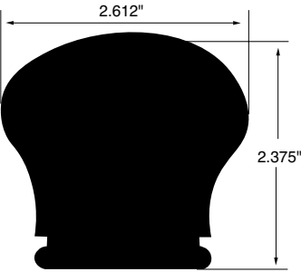
HANDRAIL WSHR9 2.612"x2.375"
