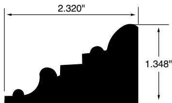
PANEL MOULDING WSPM22 2.320"x1.348"
