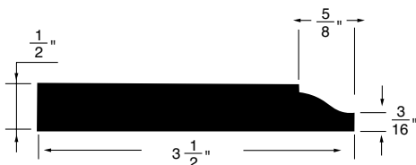
CASING WSCA39 3-1/2"x1/2"
