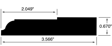
CASING WSCA46 3.566"x0.670"
