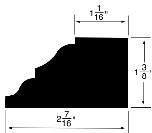
PANEL MOULDING WSPM30 2-7/16"x1-3/8"
