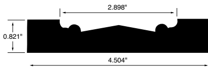
CASING WSCA7 4.504"x0.821"
