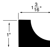
SCOTIA (CAP) MOULDING WSCM12
