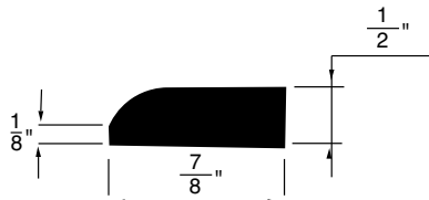
DOOR STOP WSDS3 7/8"x1/2"
