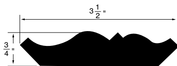
CROWN MOULDING WSCR19 - Bottom 3-1/2" x 3/4"
