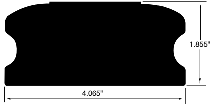
HANDRAIL WSHR8 4.065"x1.855"
