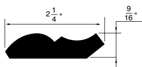
CROWN MOULDING WSCR22 2-1/4" x 9/16"
