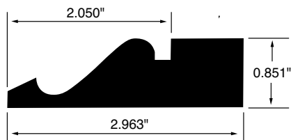
PANEL MOULDING WSPM27 2.963"x0.851"
