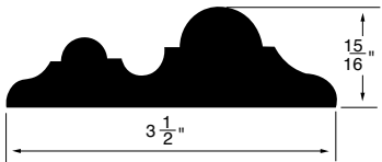
CASING WSCA22
