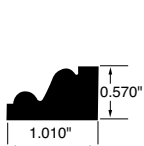
CAP MOULDING WSCM16 1.010"x0.570"
