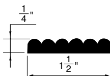
BEADED PANEL WSPM17 1/4"
