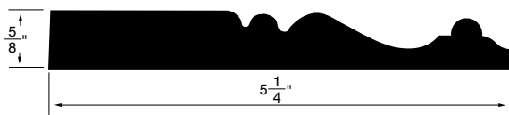
CASING WSCA44 5-1/4"x5/8"
