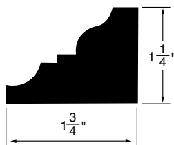
PANEL MOULDING WSPM21 1-3/4"x1-1/4"
