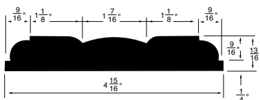
CASING WSCA6 4-15/16"x13/16"
