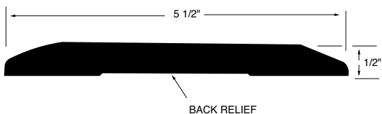
SADDLE WSSADDLE1 5-1/2"x1/2"
