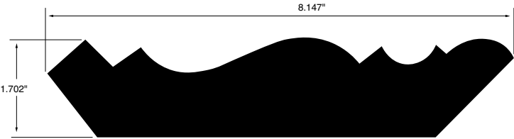
CROWN MOULDING WSCR1 8.147"x1.702"
