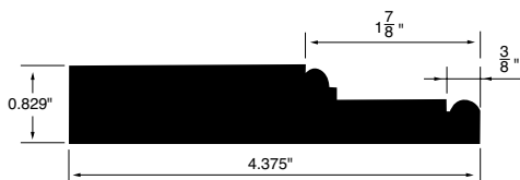
CASING WSCA14 4.375"x0.829"
