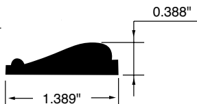
PANEL MOULDING WSPA2 1.389"x0.388"
