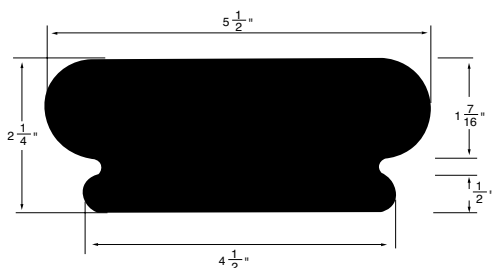
HANDRAIL - NORTH TOP RAIL WSHR17 5-1/2"x2-1/4"
