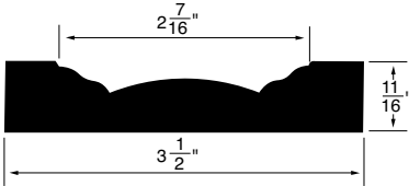
CASING WSCA50 3\frac{1}{2}" \times \frac{11}{16}"
