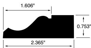
PANEL MOULDING WSPM9 2.365"x0.753"
