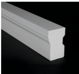
BMPVC Brick Moulding 1-1/4" X 2" X 17' All Locations
